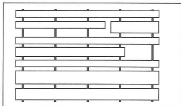
Figure 25: Stacking and Stickering of lumber
