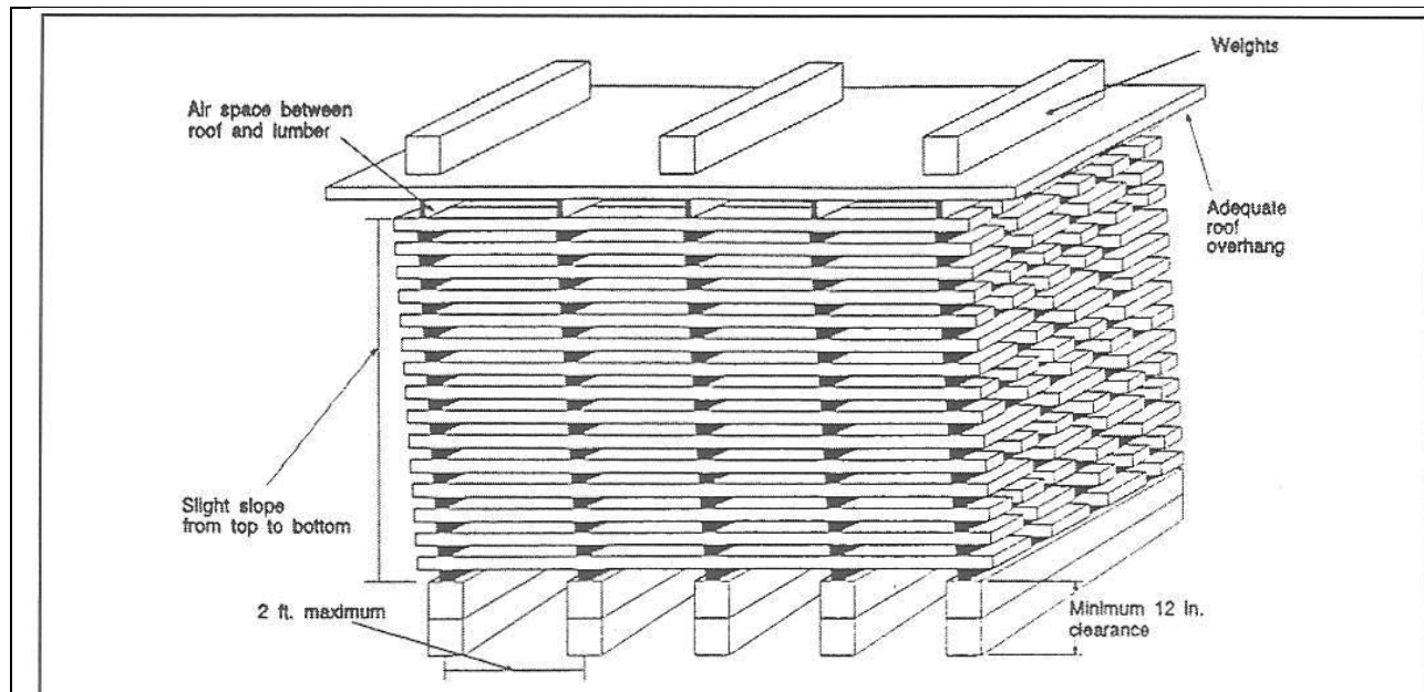
Lumber properly stacked for air drying.
