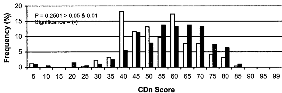
Figure 12. Score distribution pattern of tree crown density in Jambi (white bar) and P.Laut (black bar) natural forest
