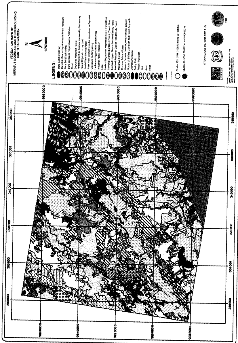
Figure 4. Vegetation Map of Meratus Mountain and Its Surrounding South Kalimantan
