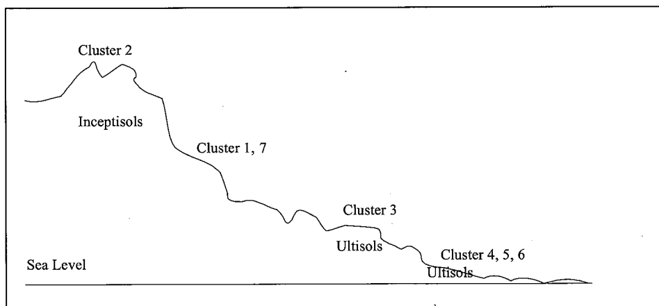
Fig. 2. Schematic topographical position of FHM cluster plots in Pulau Laut
