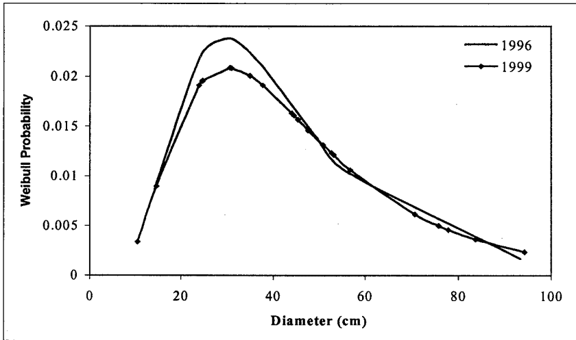
Figure 5. Probability density function of Weibull distribution for diameter of Shorea polyandra in cluster 2 Pulau Laut
