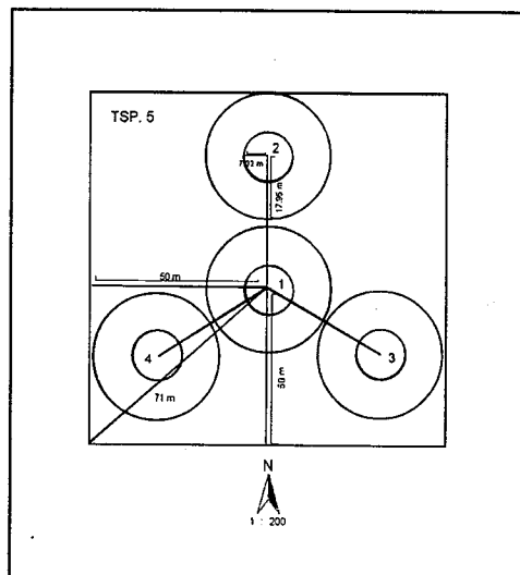
Figure 3. The Overlaid FHM Plot on NFI Permanent Sampling Plot (PSP)
