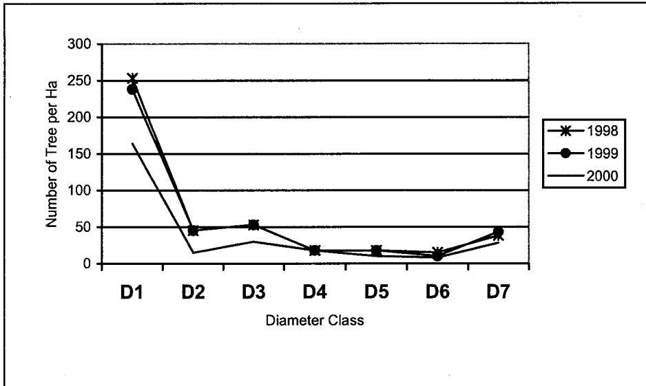
Figure 2. Diameter distribution at natural forest logged in 1978 (Cluster 1), Pulau Laut Notes: D1 = 10 cm – 19.9 cm; D2 = 20 cm – 29.9 cm; D3 = 30 cm – 39.9 cm; D4 = 40 cm – 49.9 cm; D5 = 50 cm – 59.9 cm; D6 = 60 cm – 69.9 cm; D7 = > 70 cm
