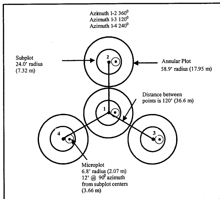
Figure 1. FHM plot layout is designed around four points (subplot centers)
