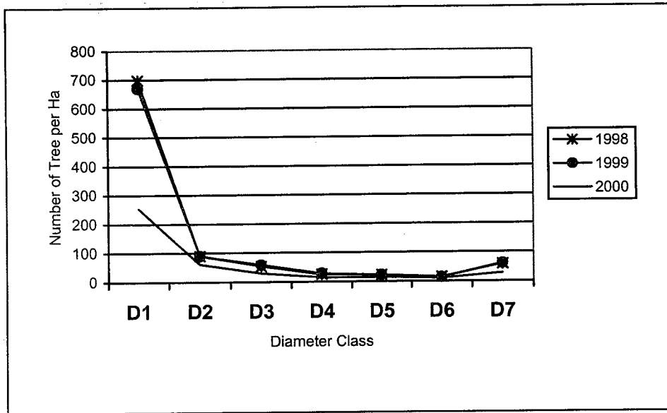
Figure 8. Diameter distribution at logged forest in 1978 (Cluster 7), Pulau Laut Notes: D1 = 10 cm – 19.9 cm; D2 = 20 cm – 29.9 cm; D3 = 30 cm – 39.9 cm; D4 = 40 cm – 49.9 cm; D5 = 50 cm – 59.9 cm; D6 = 60 cm – 69.9 cm; D7 = > 70 cm
