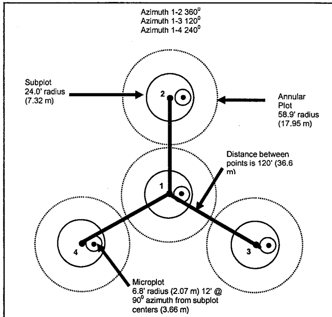
Figure 1. Four FHM plots arrangement of a cluster
