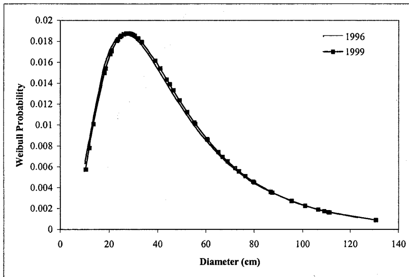
Figure 8. Probability density function of Weibull distribution for diameter of Shorea polyandra in cluster 7 Pulau Laut
