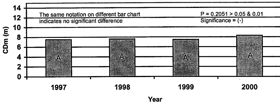
Figure 19. Change on crown diameter within the different year in Jambi natural forest, 1996 – 2000
