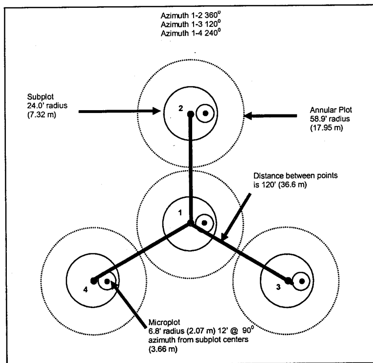
Figure 1. FHM Cluster-plot Design
