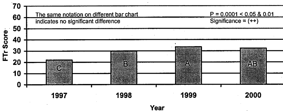
Figure 21. Change on foliage transparency within the different year in Jambi Natural Forest, 1996 - 2000
