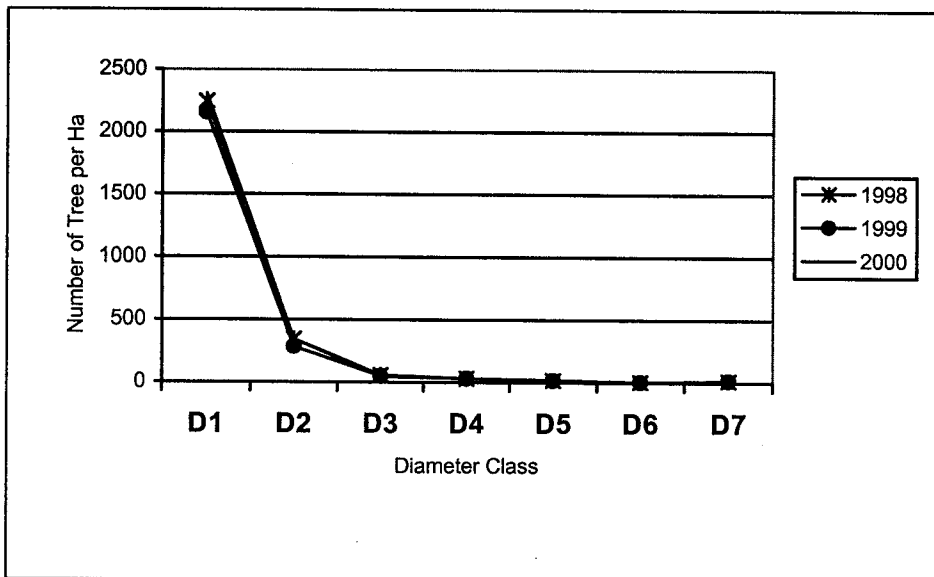
Figure 11. Diameter distribution at seed production area (Cluster 3), Jambi
