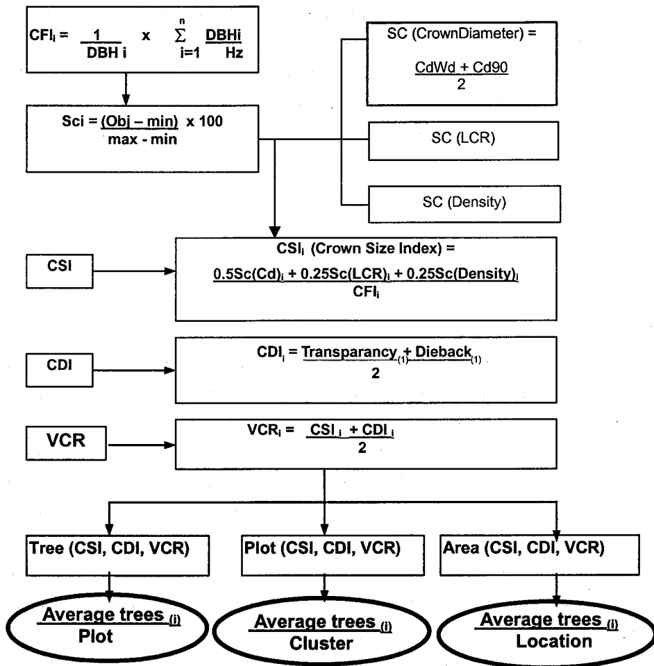
Figure 18. A crown data simplification stepping procedure in USDA FHM project
