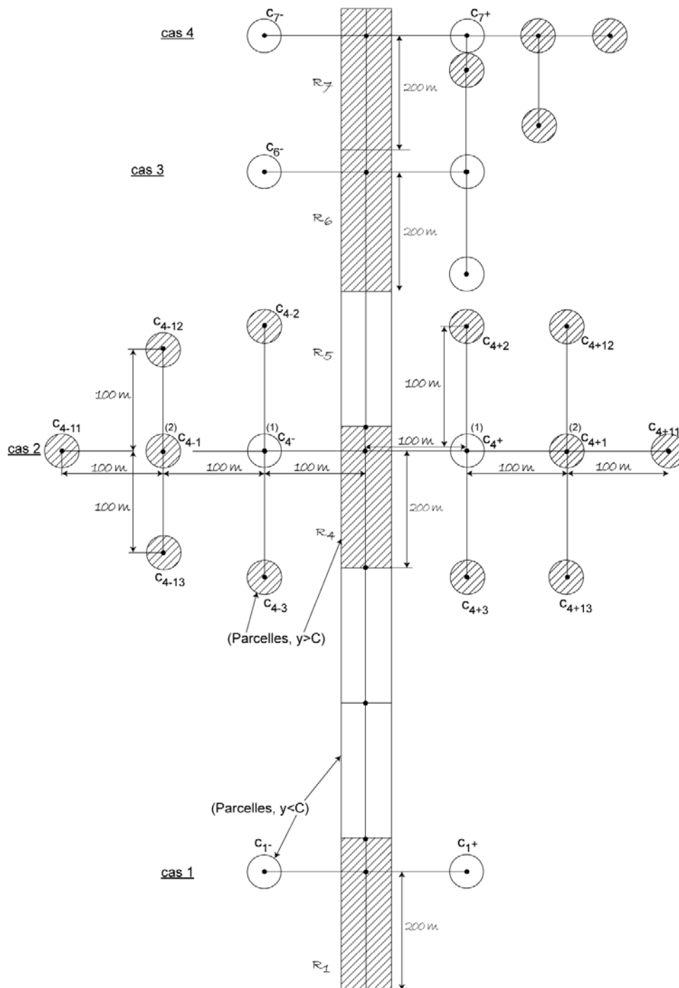
Figure 4: Sampling design of the ACS method
