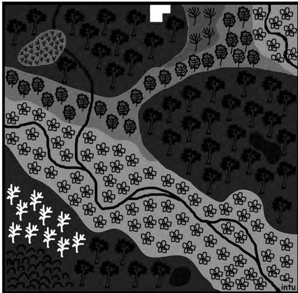
Figure 4. Schematic depiction of a forest landscape
